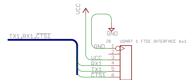
USART1 - FTDI Standard.
